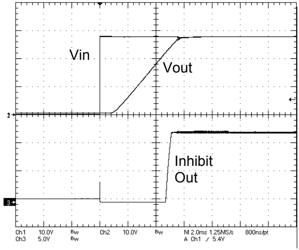
Figure 5 – Vin, Vout, Inhibit Out during turn-on at 28V
