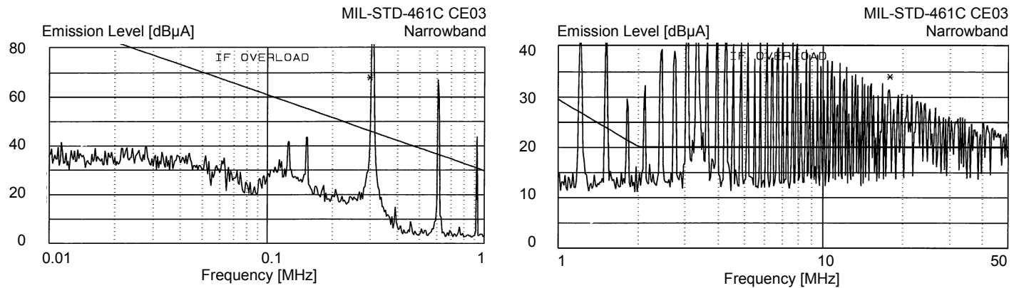
Figure 13 – 5V input line, DVPL, C_{IN}=300\mu F
