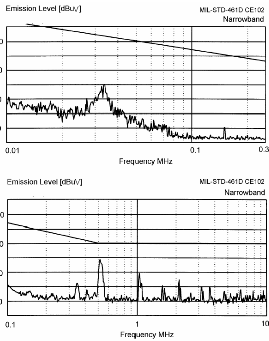
Figure 12 – MIL-STD-461D DVETR2800S
