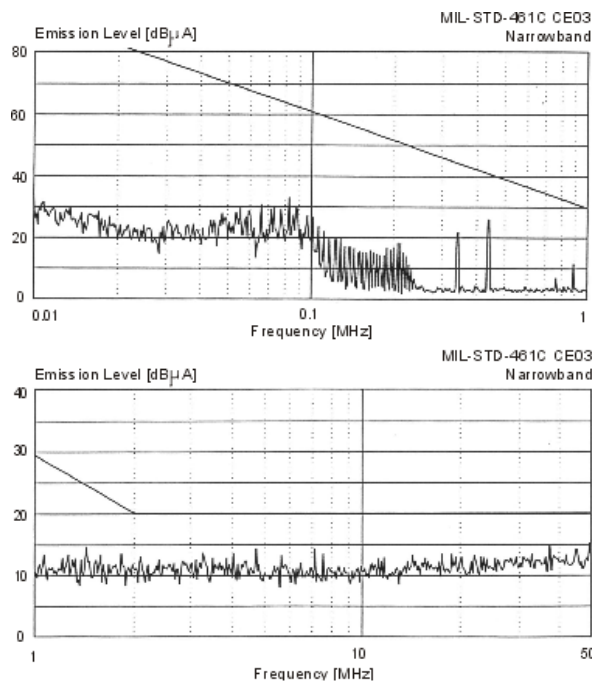
Figure 12 – SVSA2800D with EMI Filter
