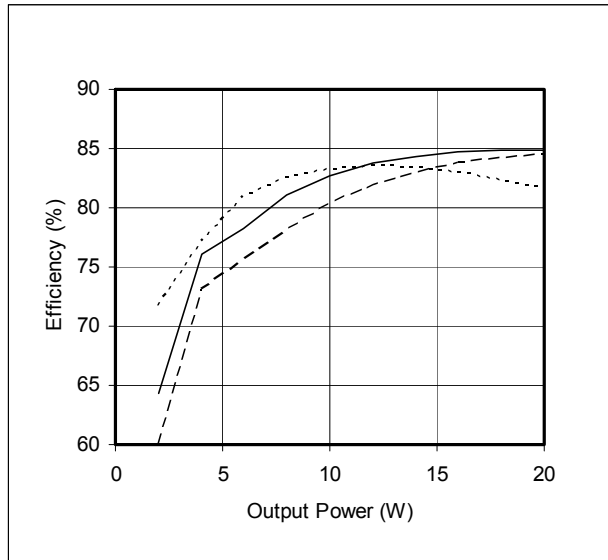
Figure 12 – SVHF2828S Efficiency (%) vs. Output Power (W)
