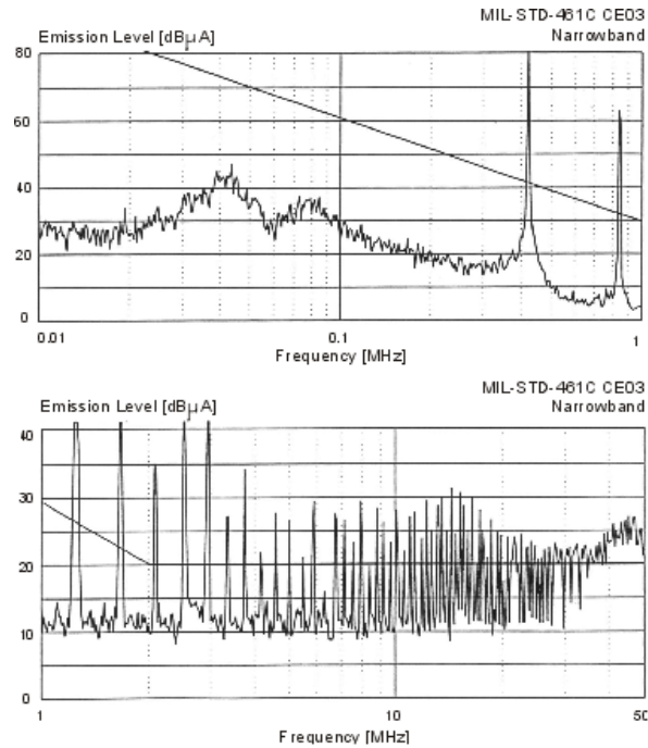
Figure 13 – SVHF2800S without EMI Filter
