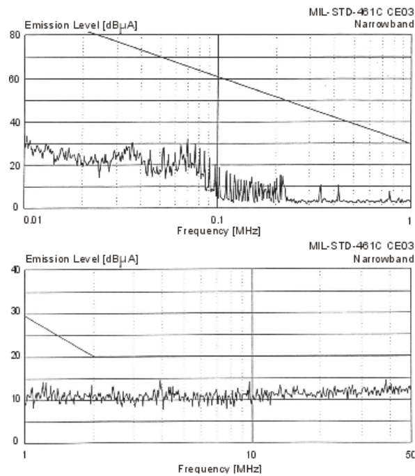
Figure 14 – SVHF2800S with EMI Filter
