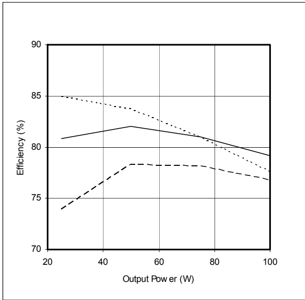
Figure 10 – SVFL2805D Efficiency (%) vs. Output Power (W)
