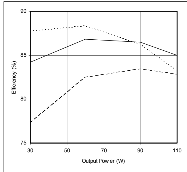
Figure 11 – SVFL2812D Efficiency (%) vs. Output Power (W)
