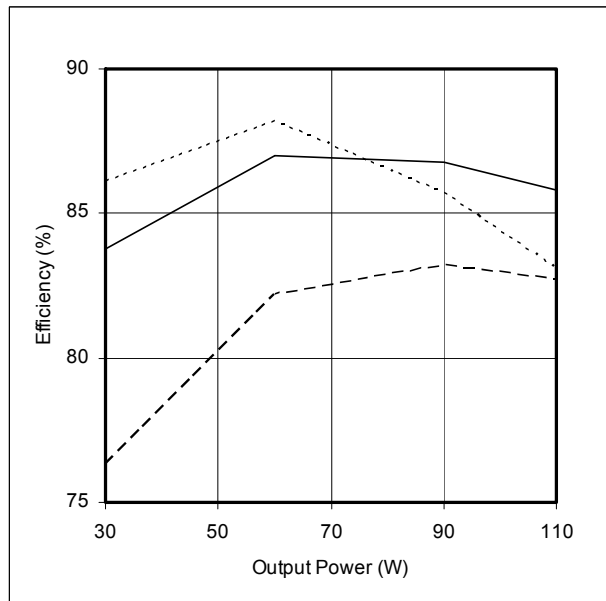
Figure 12 – SVFL2815D Efficiency (%) vs. Output Power (W)
