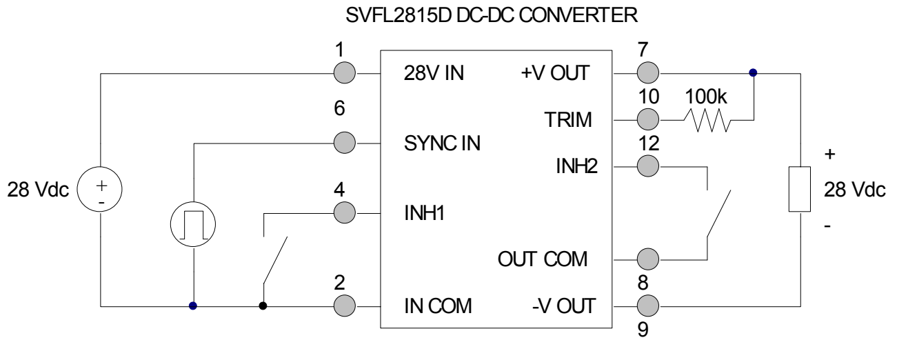
Figure 6: +28 Volt Output Converter Using SVFL2815D Converter
