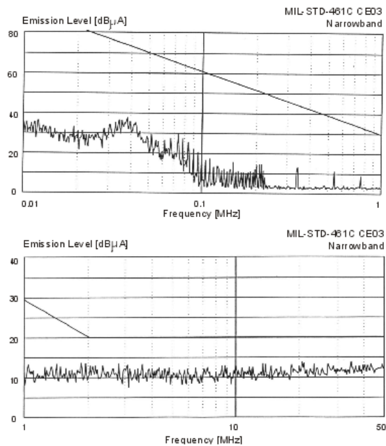
Figure 14 – SVFL2800D with EMI Filter
