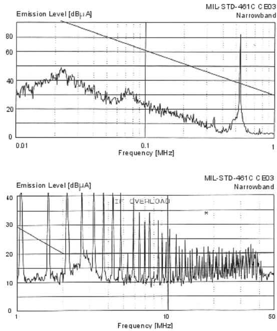
Figure 13 – SVFL2800D without EMI Filter
